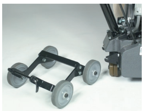
The patented Dolly Transport™ system makes transporting the FloorCrafter to job sites easier than ever.
